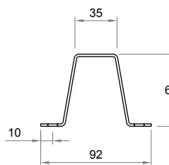
OMG.060 Profile Omega 60 mm
