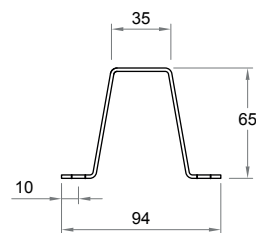
OMG.065 Profile Omega 65 mm
