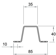
OMG.040 Profile Omega 40 mm
