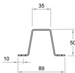
OMG.050 Profile Omega 50 mm
